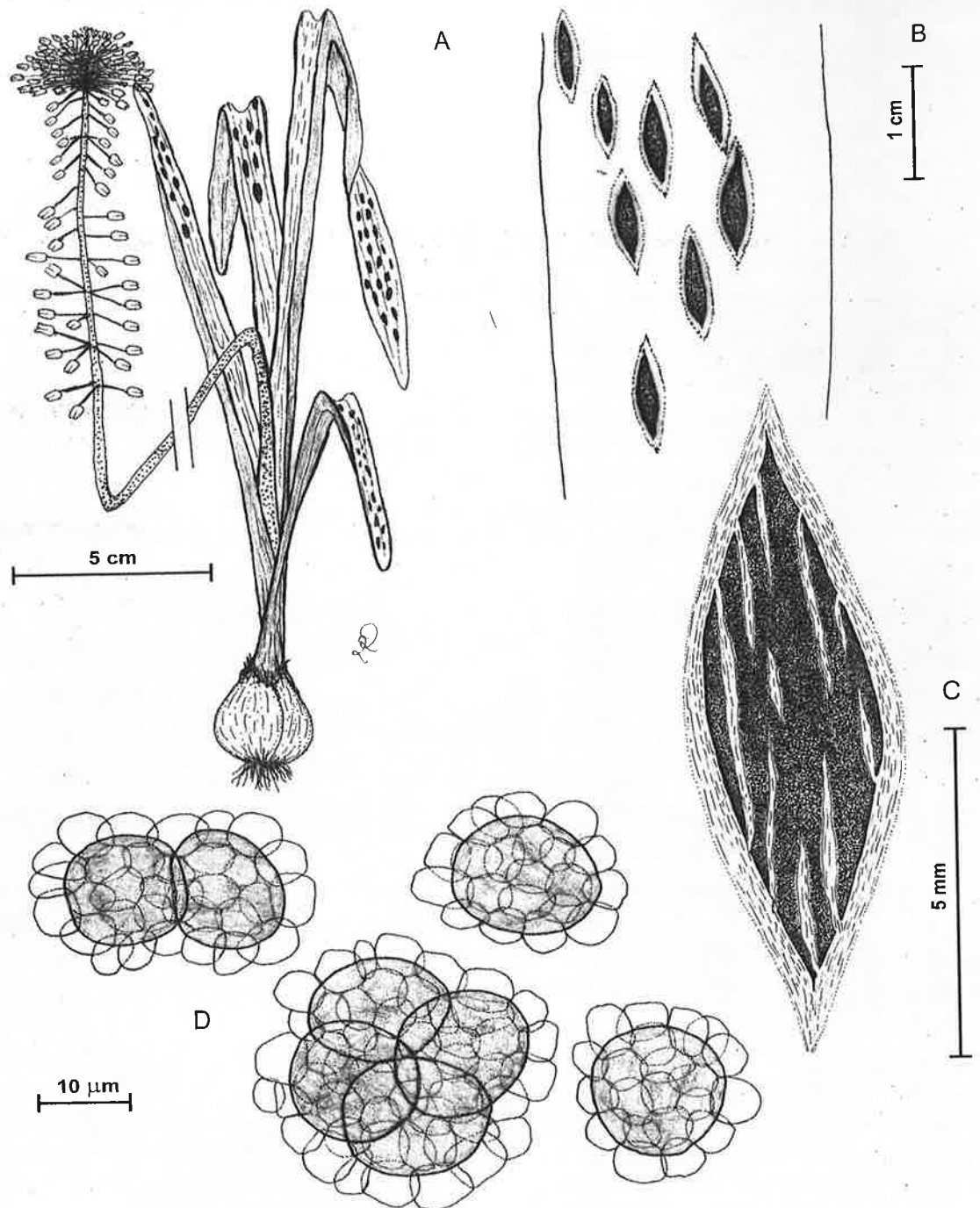
Fig. 1. Urocystis muscaridis (Niessl) Moesz on Muscari comosum (L.) Mill. A - infected host; B - sori in leaf, C - sorus, D - spore balls.
